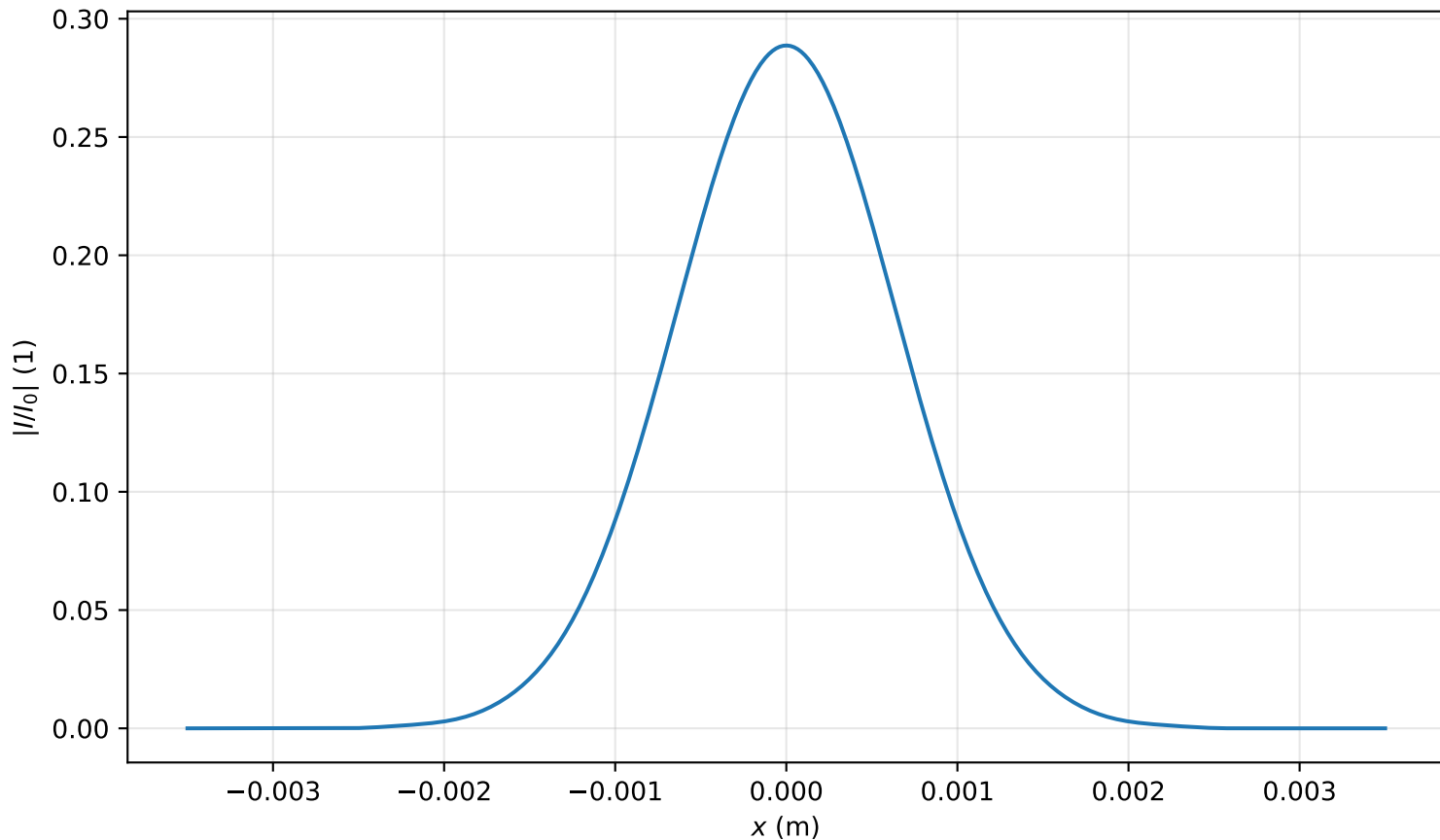
Intensity profile I(x, y = 0, z = 3.344m)/I_0 , P_{in}=0.1P_{cr} , artificial time
